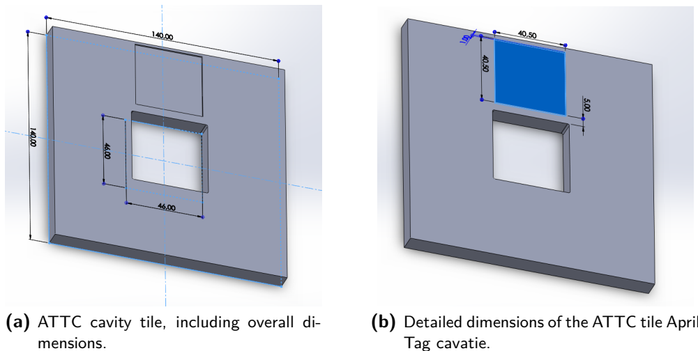
Figure 3.20: 3D construction of the ATTC Precision Placement cavity tile.
