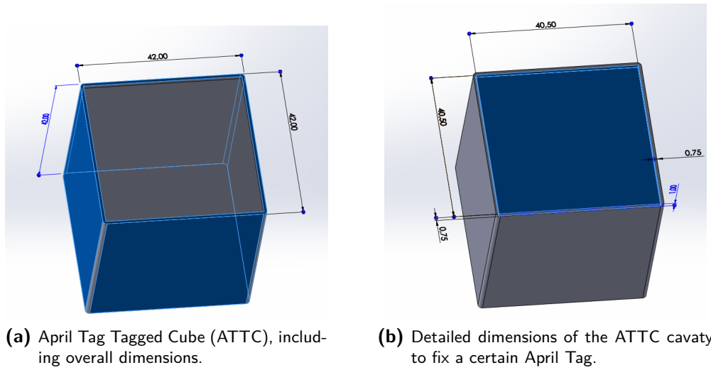
Figure 3.19: 3D construction of the ATTC as manipulation object.
