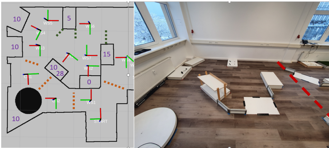
Figure 8.1: Example Arena for a small VRC Setup — Left: Annotated map - Right: Real Image
