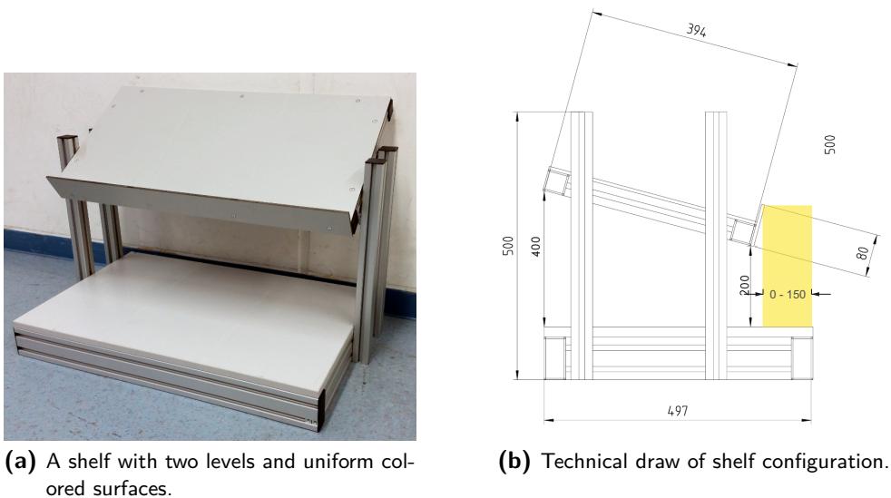
Figure 3.7: Exemplary shelf and generic technical drawing.
