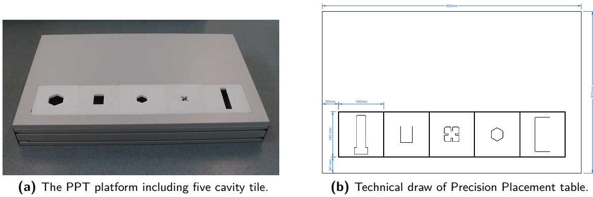
Figure 3.10: Exemplary Precision Placement table and generic technical drawing.
