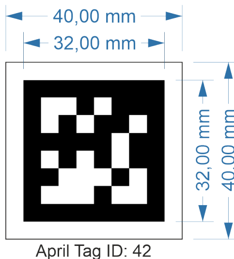
Figure 3.18: Example of an April Tag with the ID 42. Encoding is from the 36h11-April Tag Family.
