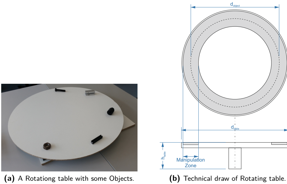
Figure 3.8: Exemplary Rotating table and generic technical drawing.
